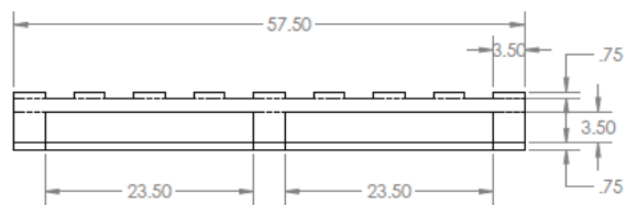
Figure 3 Dimensions of the short side of the pallet
