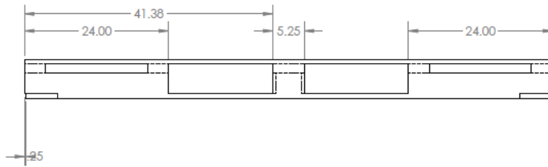
Figure 2 Dimensions on the long side of the pallet
