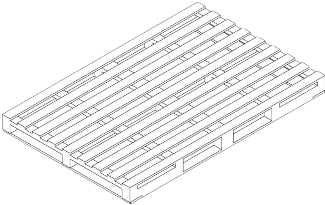
Figure 1 Schematic of revised plate pallet for 50x80 and 50x65 plates
