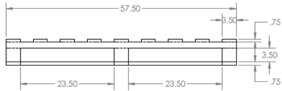
Figure 3 Dimensions of the short side of the pallet
